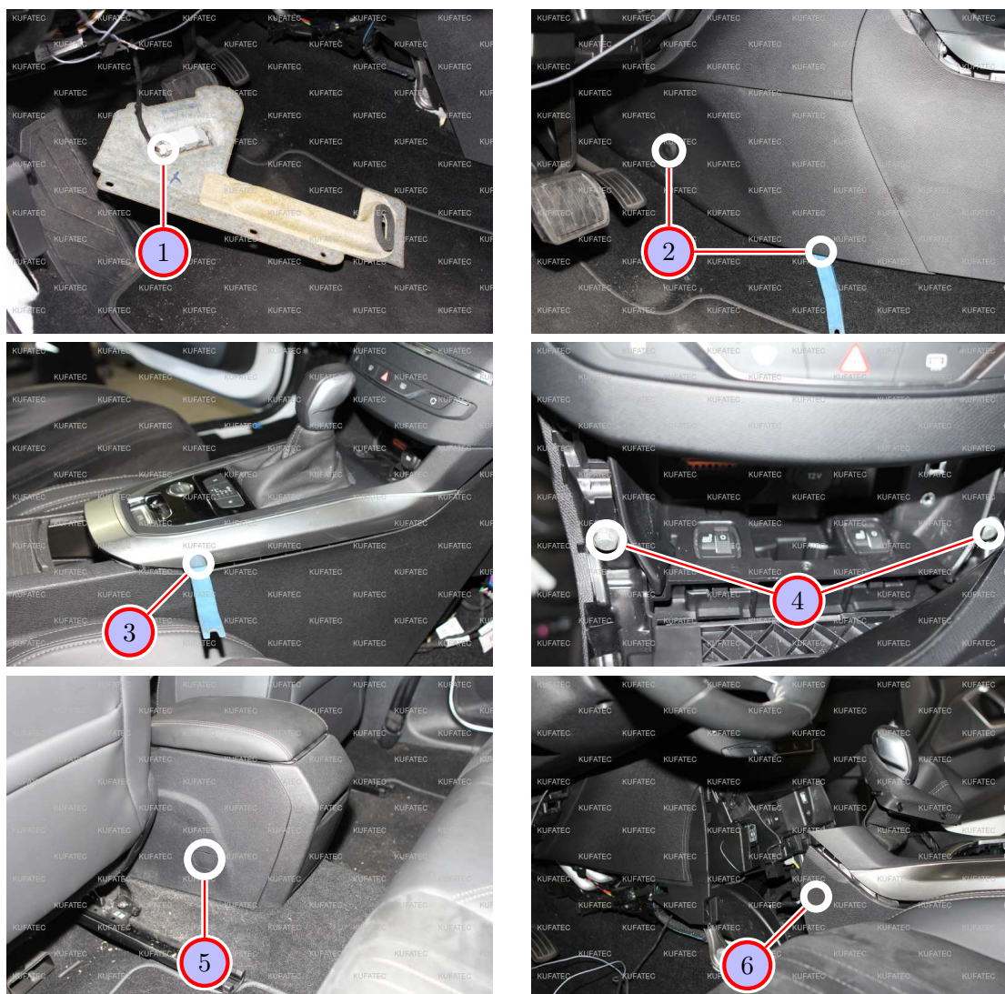
Figure 5: Removing trim panel center console
